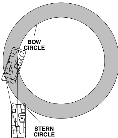
FIGURE 5-2 TURNING
