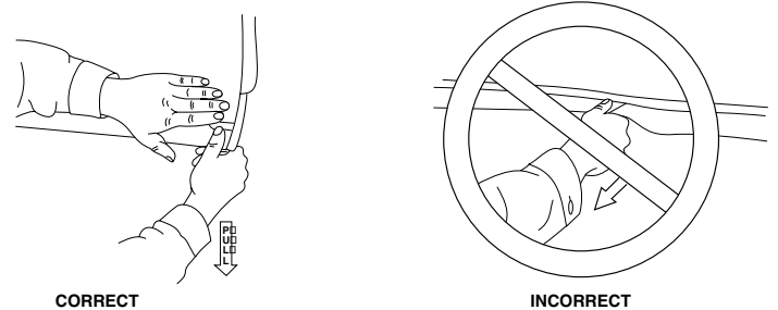
FIGURE 3-2 J-CLIP™
