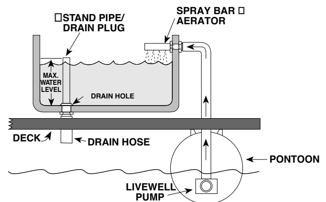
FIGURE 3-1 TYPICAL LIVEWELL
