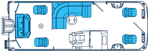
ANGLER LAYOUT offers angler station(s) , fishing chairs , L-shaped couch , and open water panels .
