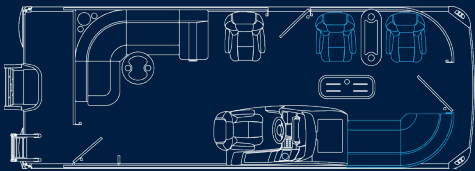
DL LAYOUT features dinette layout with bow starboard couch and port side dual chairs .
