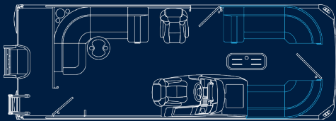
CL LAYOUT features couch layout with bow starboard and port side couches .
