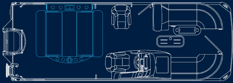
RL LAYOUT features 7-position convertible rear lounge/bed .
