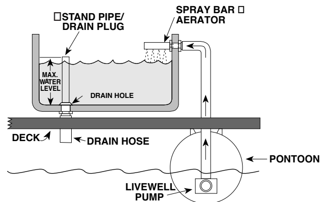
FIGURE 3-1 TYPICAL LIVEWELL
