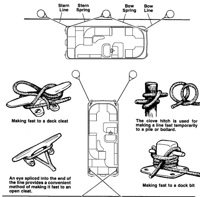
FIGURE 5-4 MOORING
