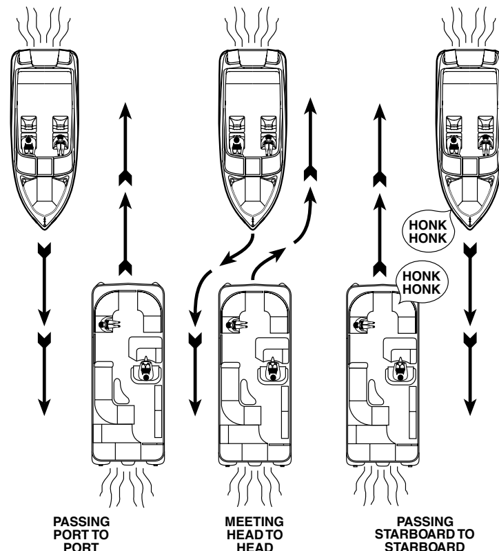
FIGURE 8-1 MEETING HEAD-ON
