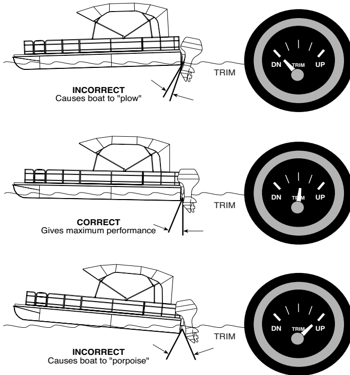
FIGURE 5-3 TRIMMING
