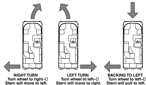
FIGURE 5-2 STEERING
