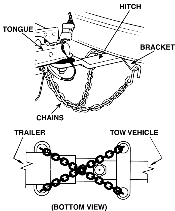
FIGURE 4-1 SAFETY CHAINS
