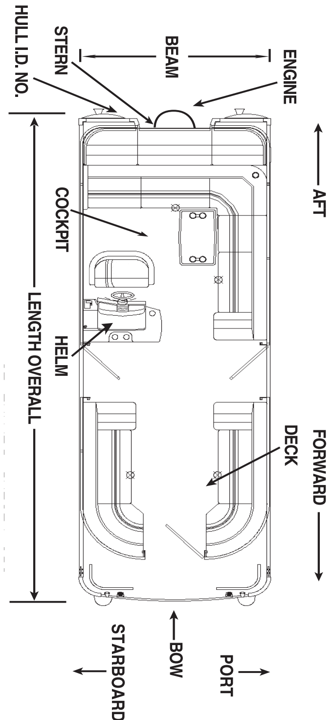
FIGURE 1-1 TERMINOLOGY
