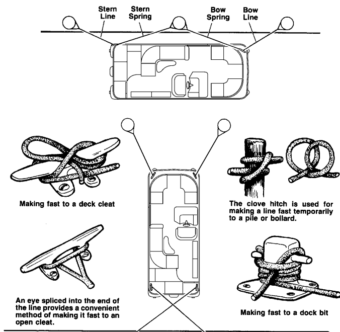
FIGURE 5-5 MOORING
