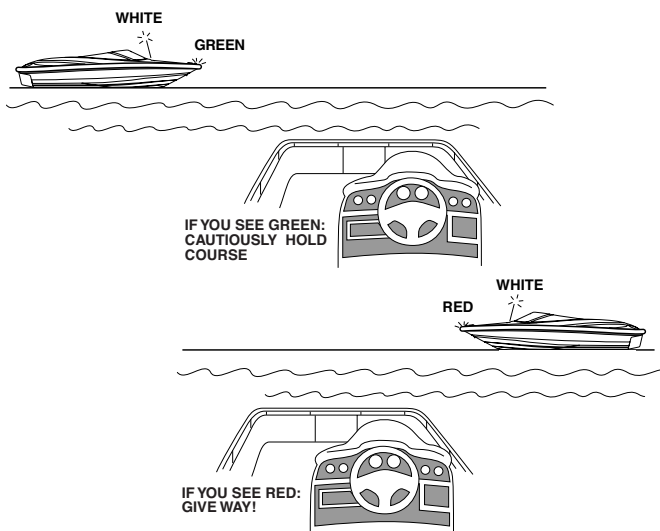
FIGURE 8-4 NIGHT RUNNING
