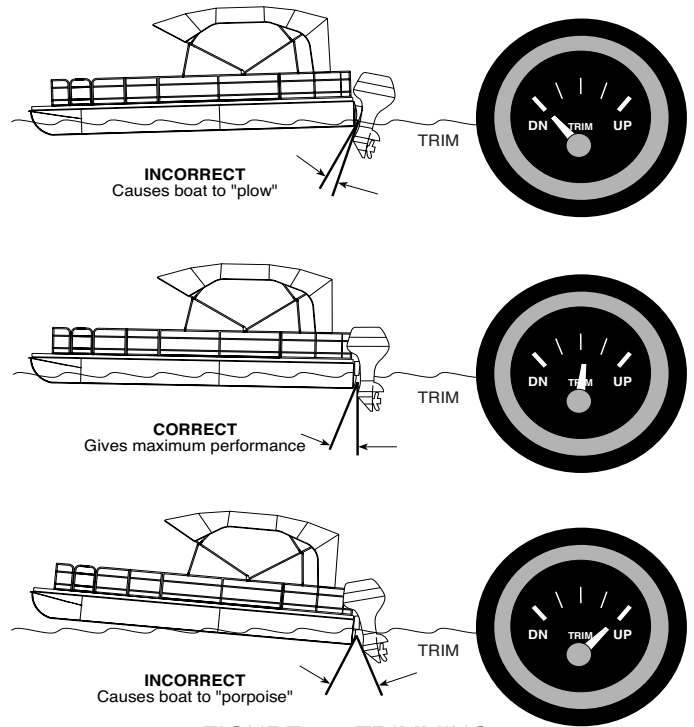
FIGURE 5-4 TRIMMING
