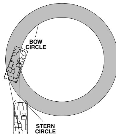
FIGURE 5-3 TURNING
